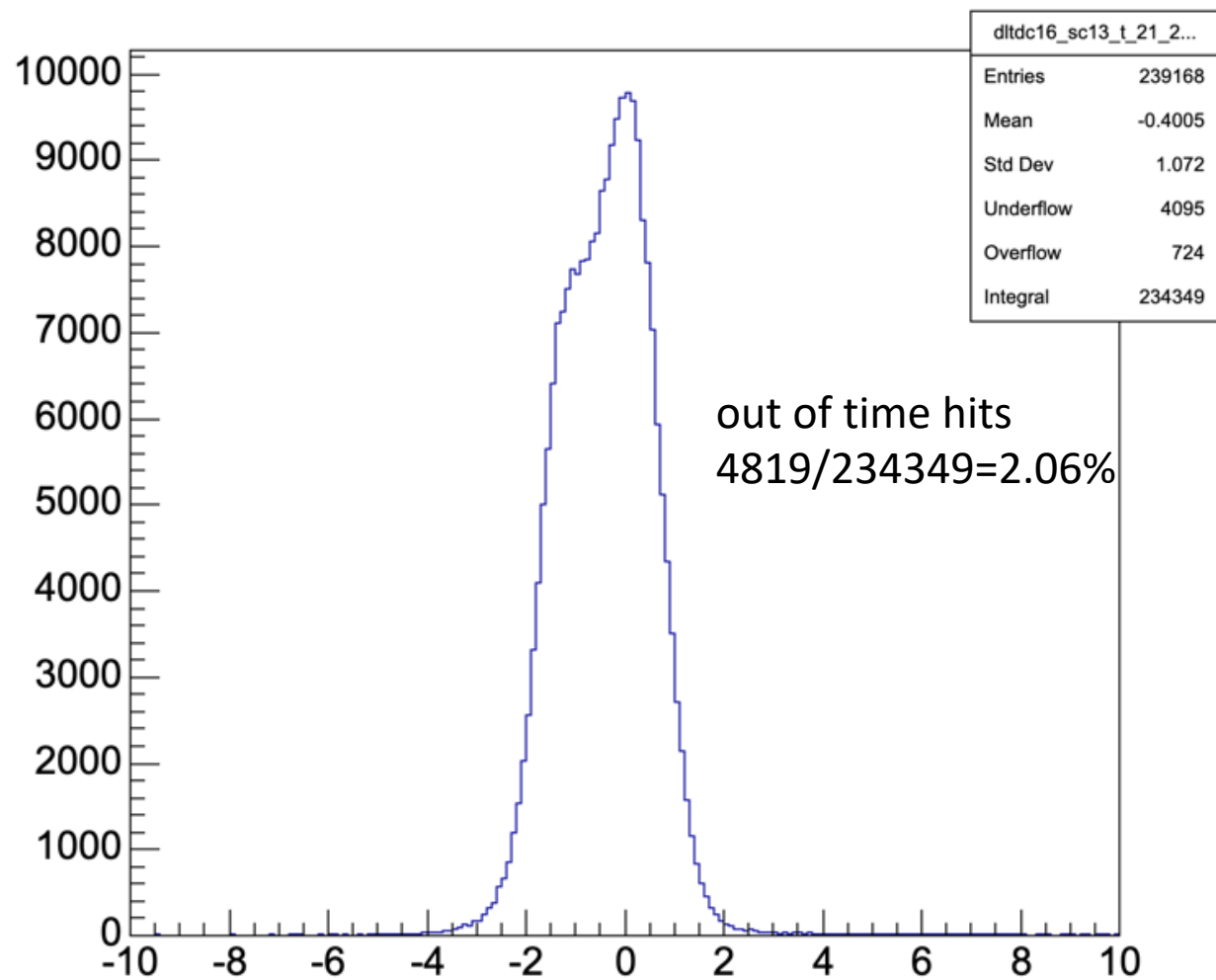
sc13 time difference ch29 minus ch21, ns
