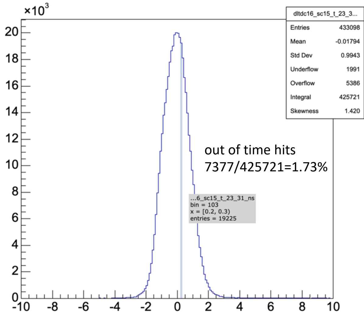
sc15 time difference ch31 minus ch23, ns
