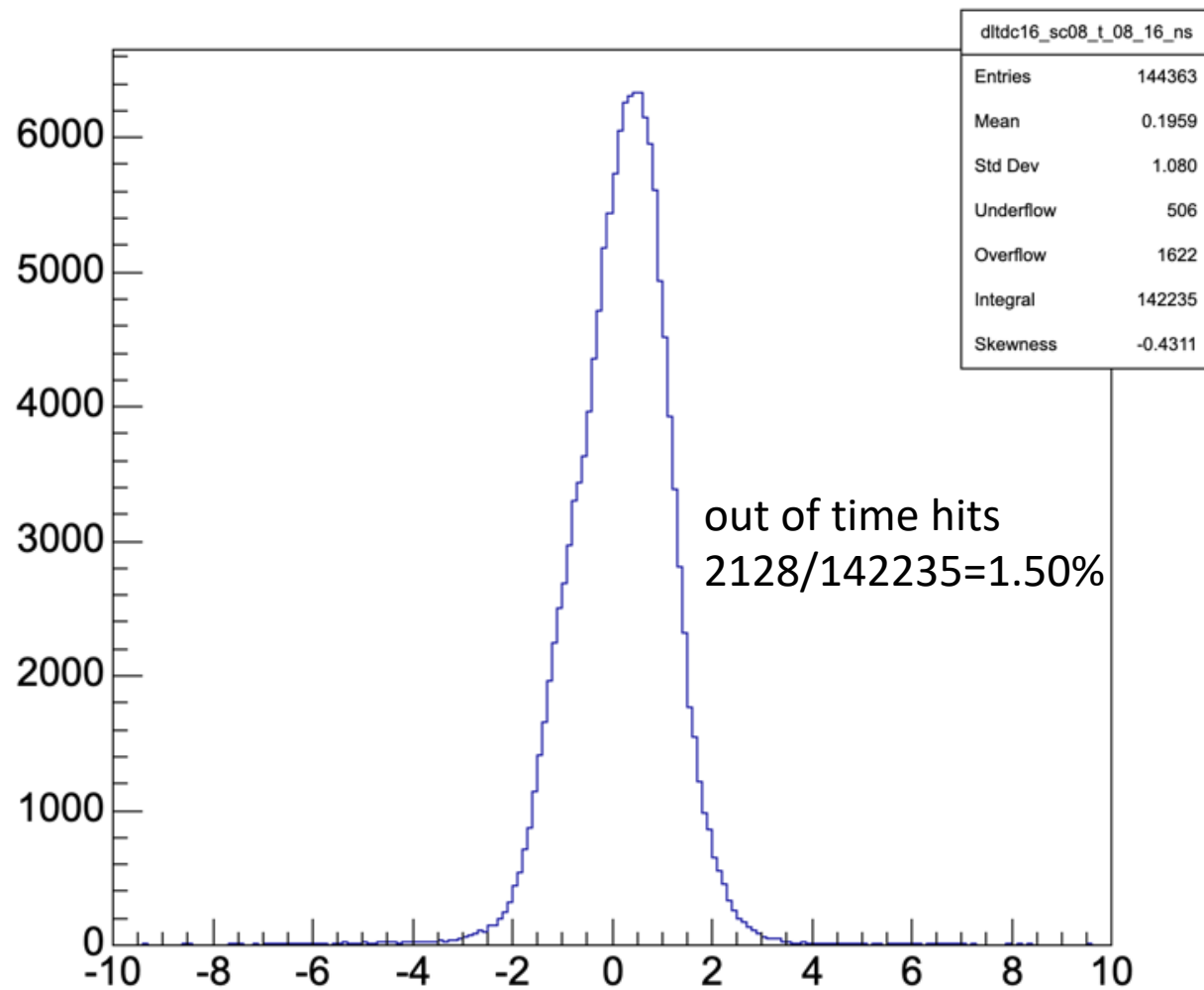
sc08 time difference ch16 minus ch08, ns
