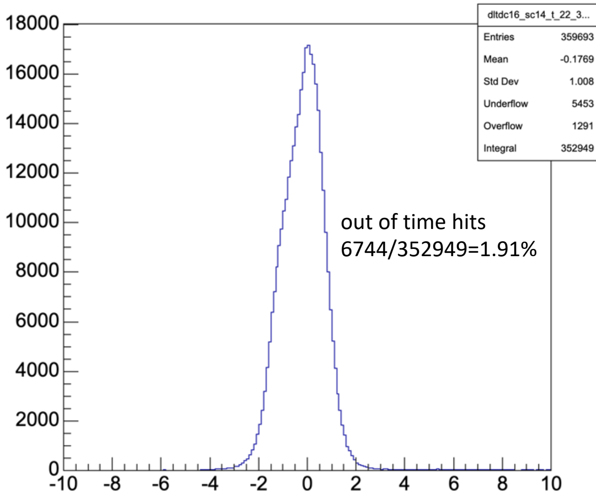
sc14 time difference ch30 minus ch22, ns
